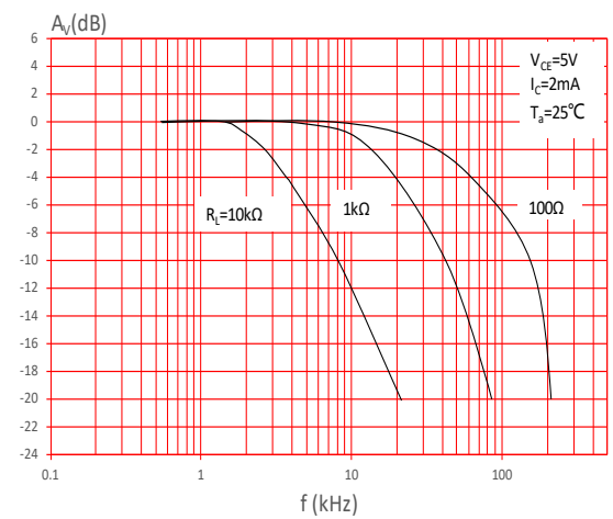
FIG.10: Frequency Response
