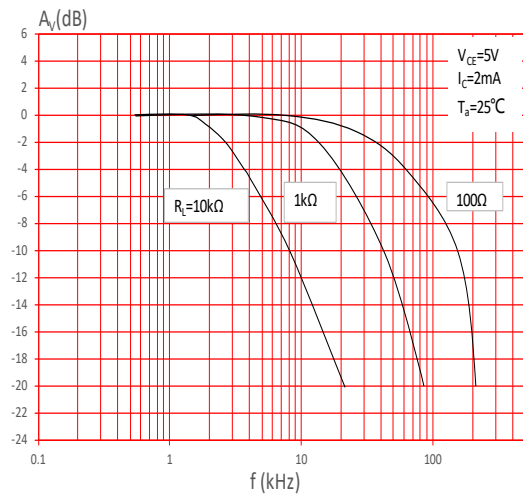
FIG.10: Frequency Response
